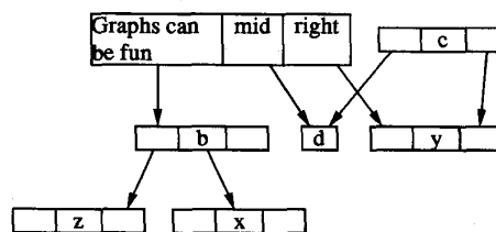
Fig. 14. Node ports in a graph.
